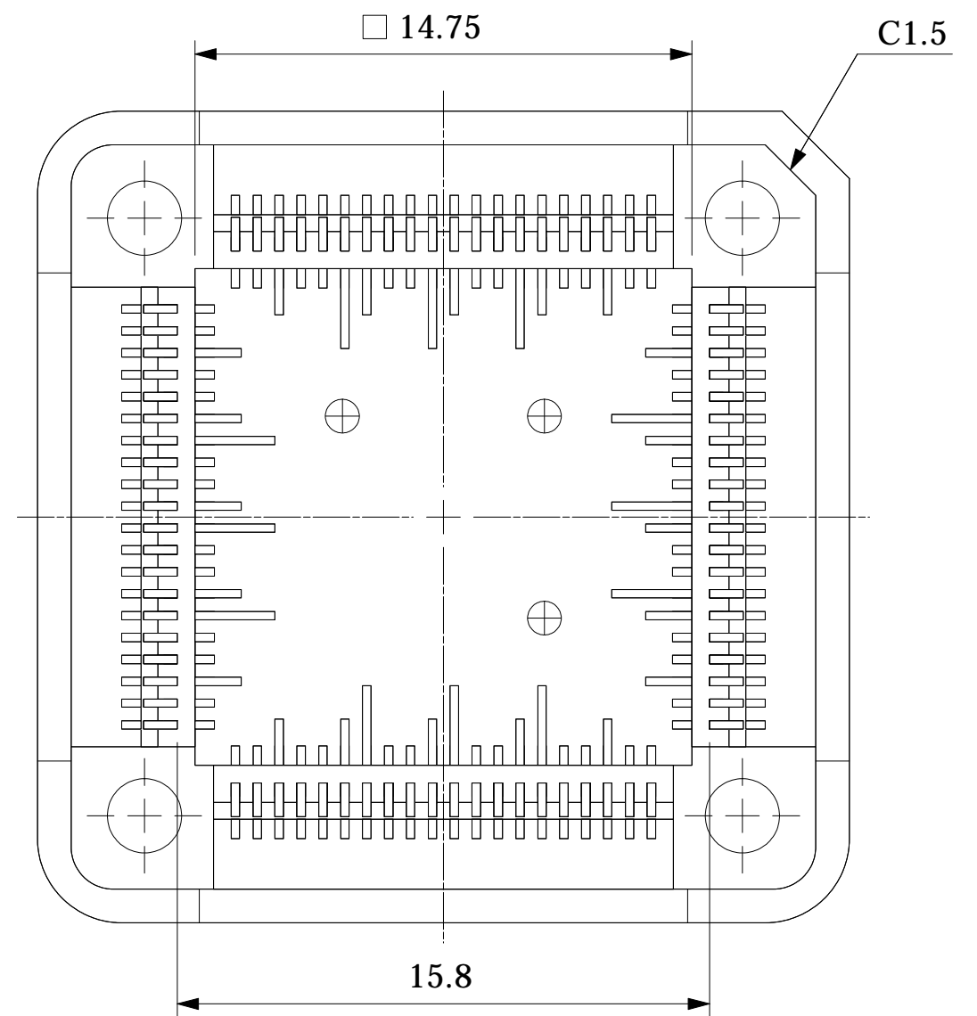
BOTTOM VIEW
