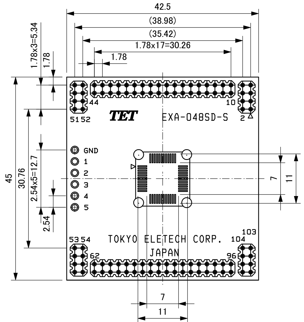
TOP VIEW
