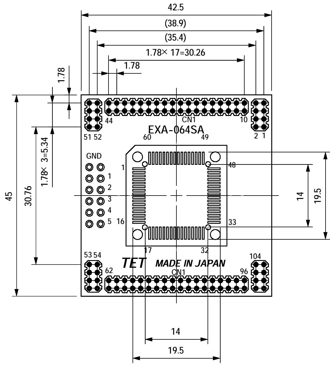
TOP VIEW
