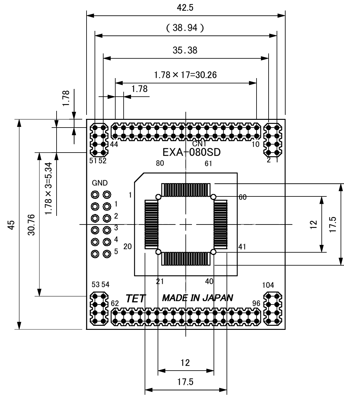
TOP VIEW
