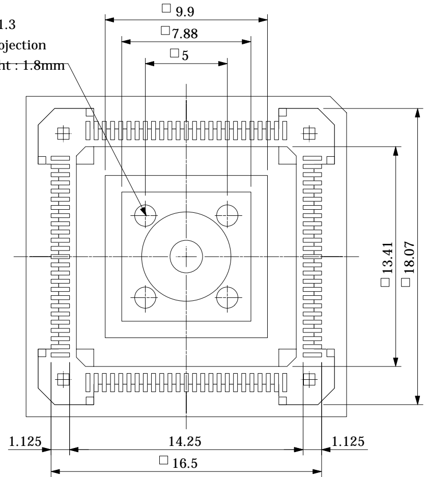
BOTTOM VIEW
