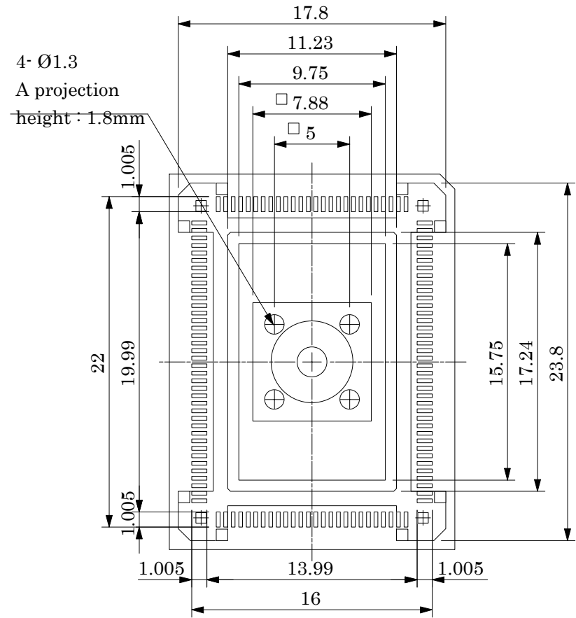
BOTTOM VIEW
