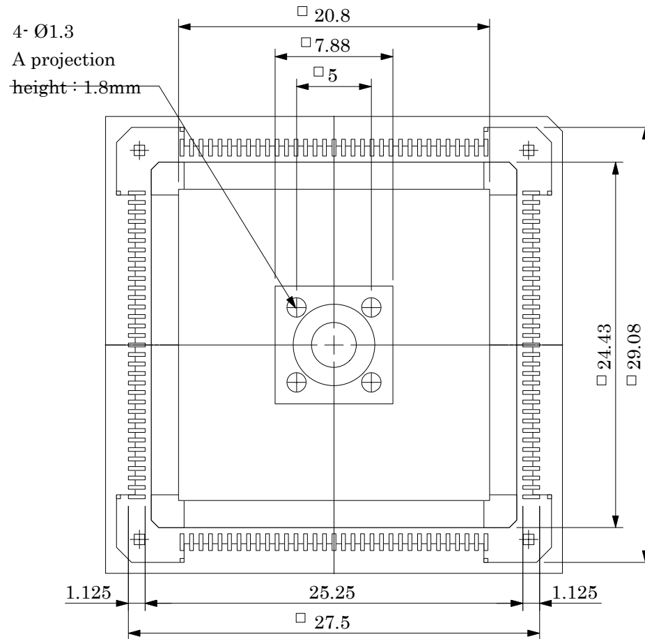
BOTTOM VIEW
