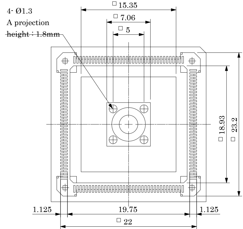
BOTTOM VIEW
